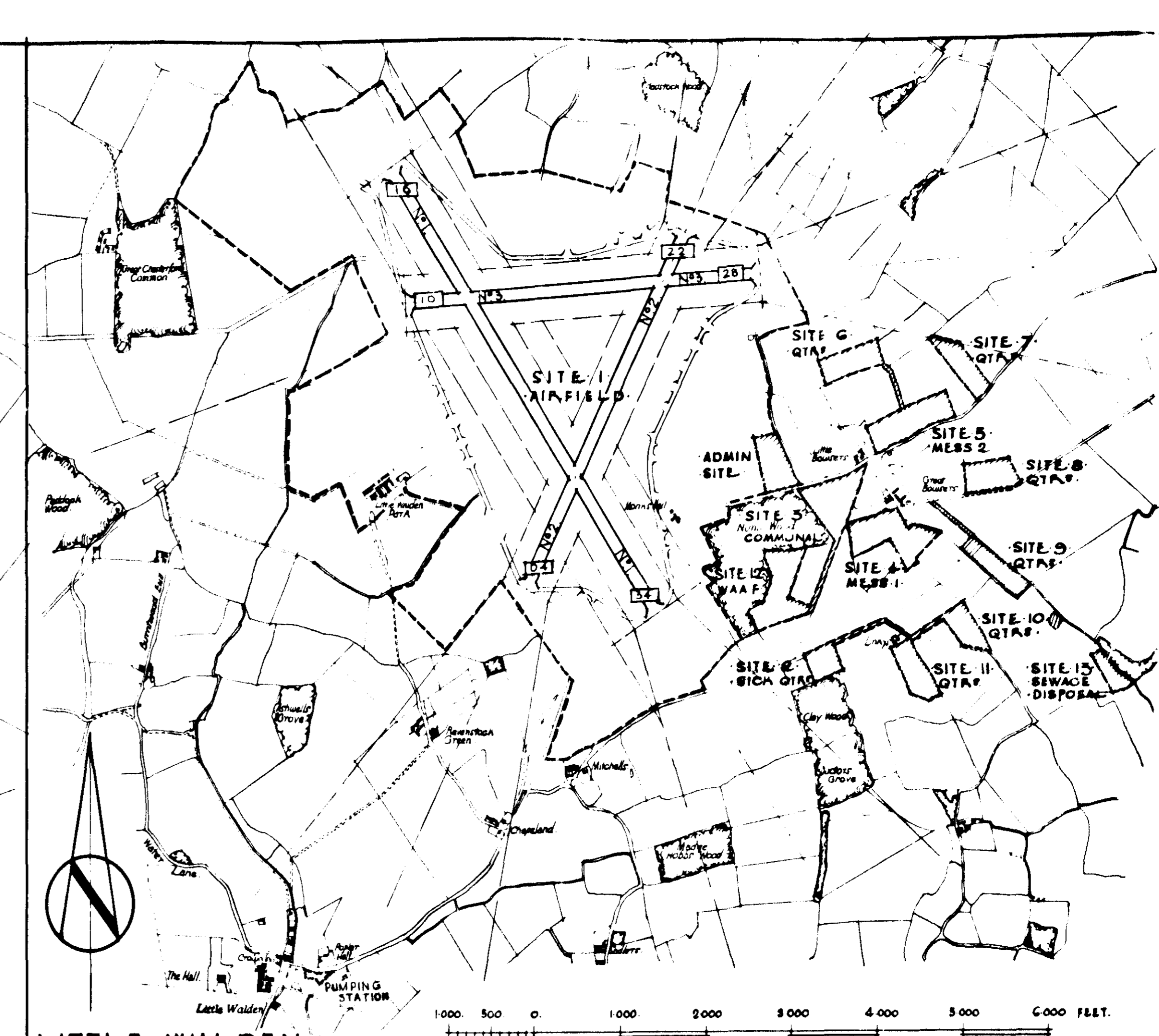
LITTLE WALDEN (HADSTOCK) LOCATION PLAN SCALE: 6" TO ONE MILE BASED ON O.S. SHEET 1:25,000 ED. 1934
