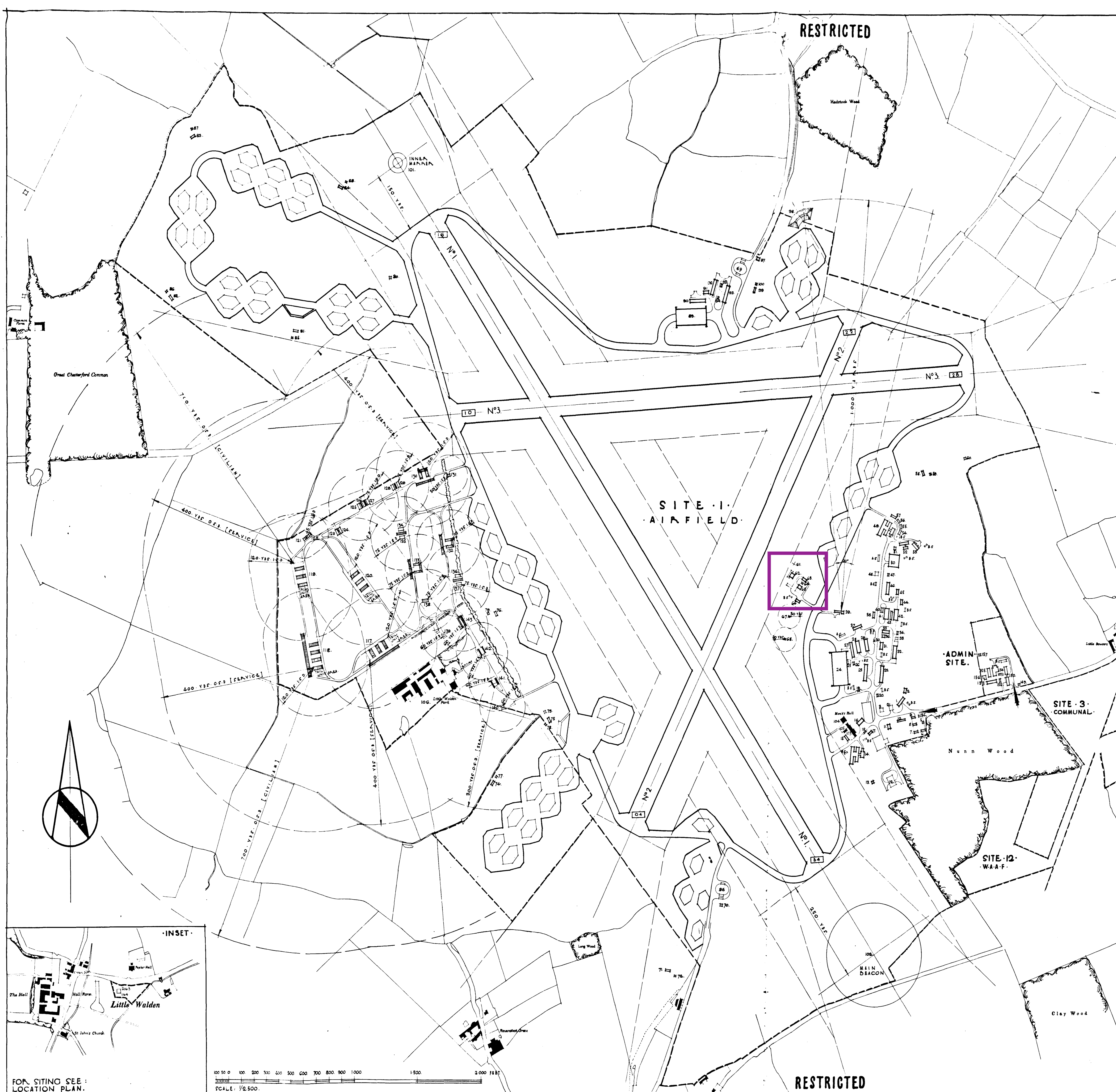
LITTLE WALDEN (HADSTOCK) LOCATION PLAN SCALE: 6" TO ONE MILE BASED ON O.S. SHEET 1:25,000 ED. 1934
